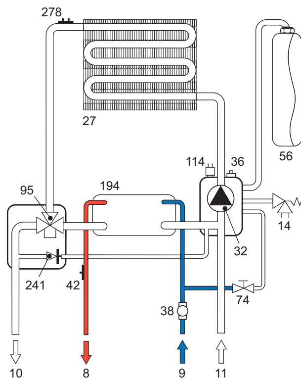
fig. 23 - DHW Circuit
