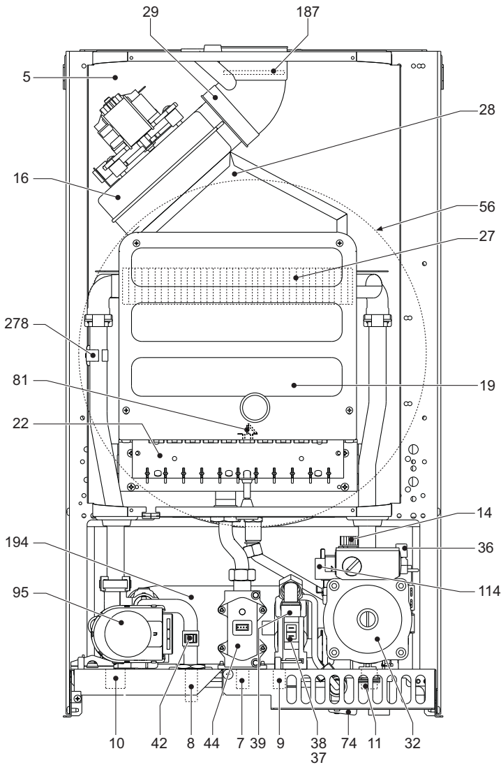
fig. 21 - Vista general CLIZIA D 24 AS
