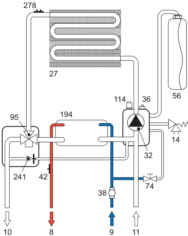
fig. 23 - Circuito de AS
