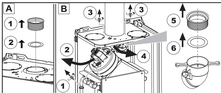
A Baffle replacement with boiler not installed
