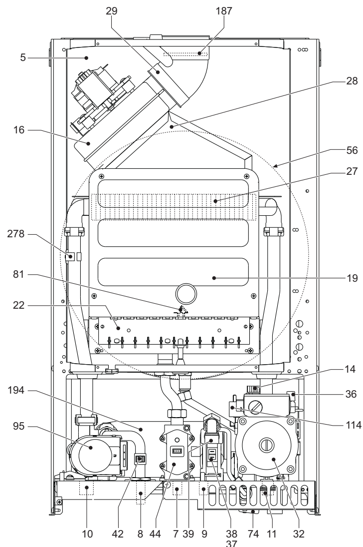
fig. 21 - General view CLIZIA D 24 AS
