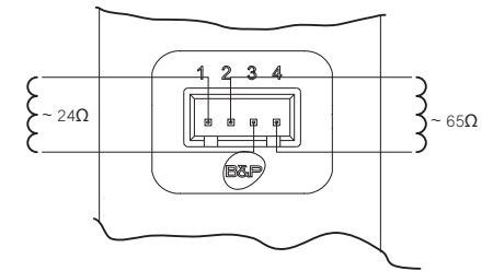
fig. 19 - Gas valve connection
