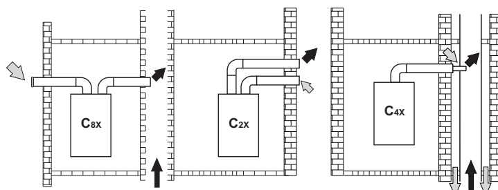
fig. 16 - Examples of connection to flues (→ = Air / → = Fumes)
